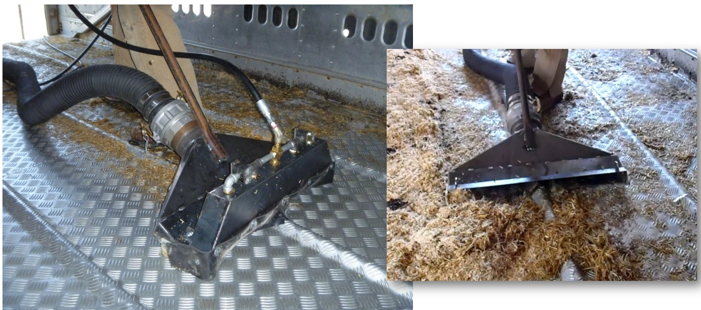
Pressure wash with vacuum ( left) compared to dry vacuum only (right) . Source: Prairie Agricultural Machinery Institute
